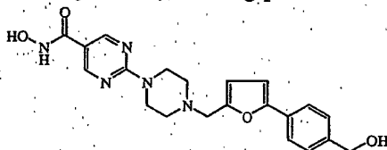
.0.83 CF 3 COOH compound 5
